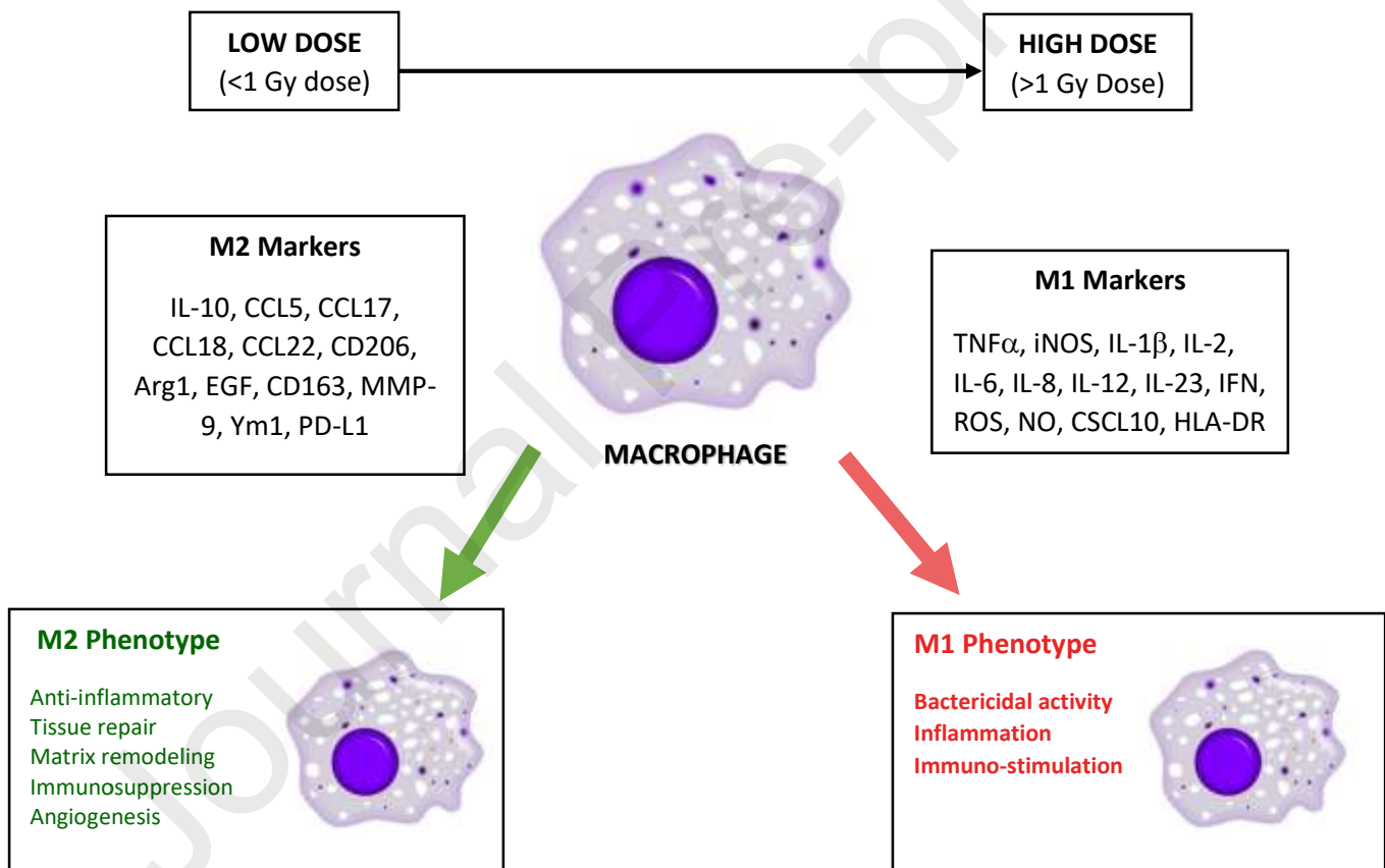
Figure 1: Radiation Dose and Macrophage Polarization (Adapted from: Genard et al 35 , Calabrese et al 37 , Pinto et al 38 )
